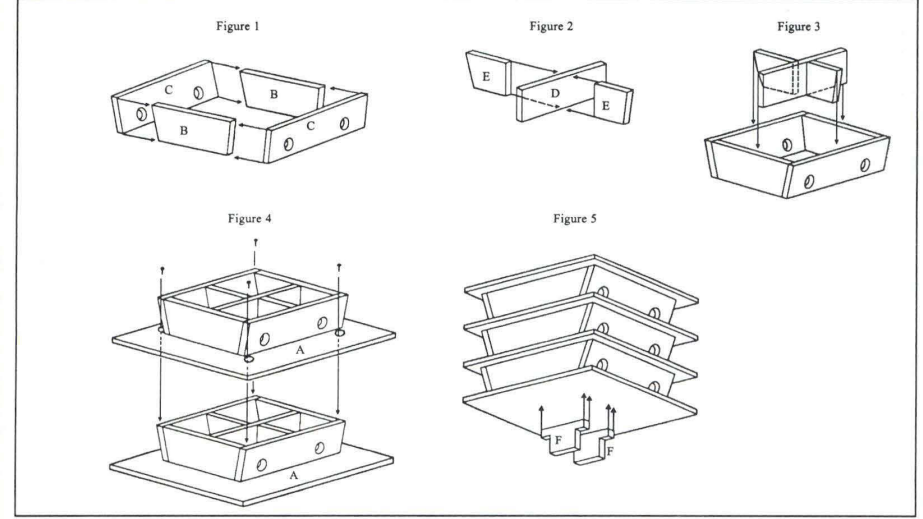
Diagram III Assembly of multi-compartment nest box
